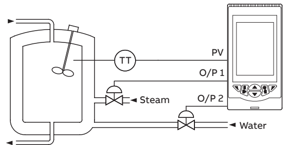
Figure 10 Split output control example
