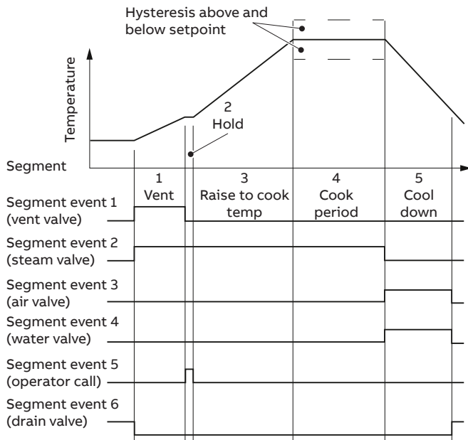
Figure 18 Profile control
