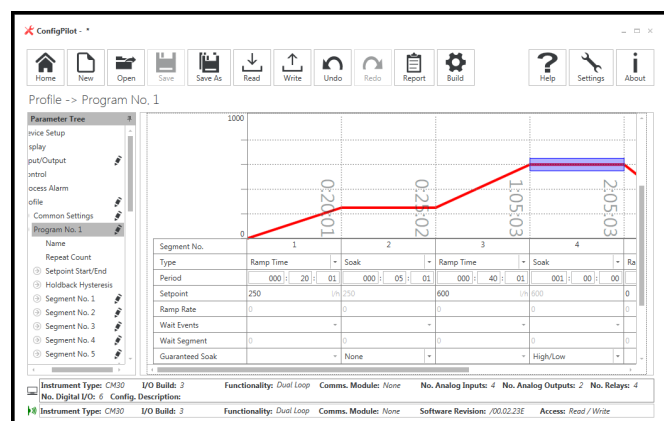
Figure 16 Profile configuration
