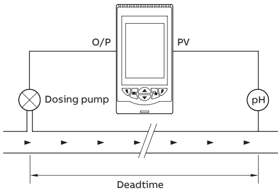
Figure 8 Predictive control example
